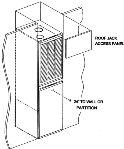
ALCOVE INSTALLATION
