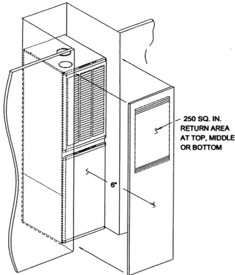
CLOSET INSTALLATION
