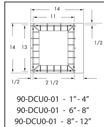
FIG. E - Duct Connector
