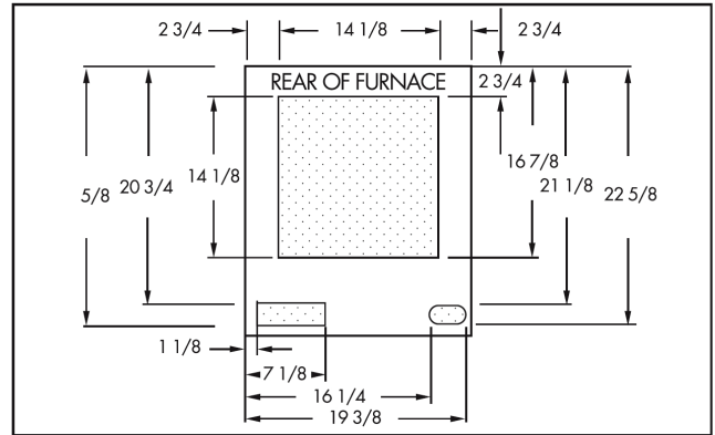
FIG.D Duct Connector Opening, Fuel & A/C Lines
