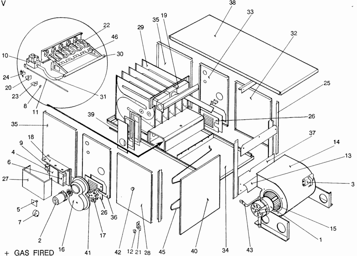
FIG. 1 - 80 + GAS FIRED HORIZONTAL FURNACES
