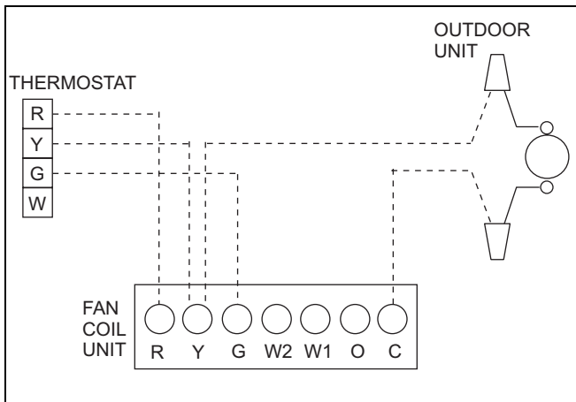
FIGURE 13 : Cooling Wiring
