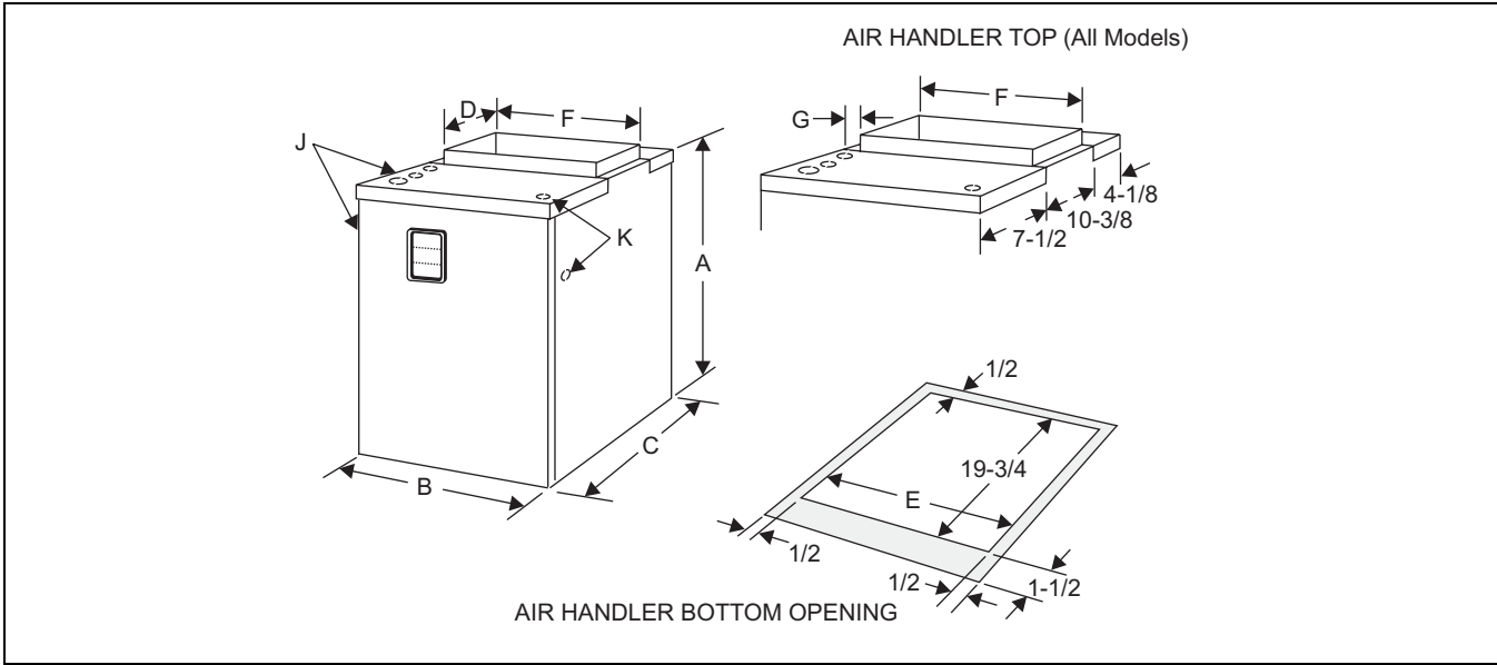
FIGURE 4 : Dimensions & Duct Sizes
