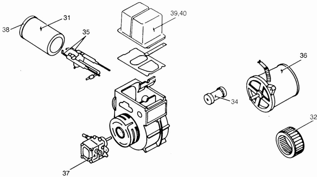
FIG. 2 - BURNER PARTS
