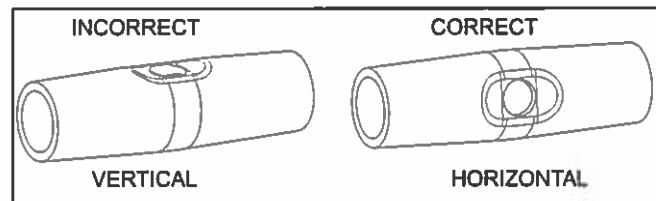
FIGURE 1: Tapped Gas Pipe Nipple
